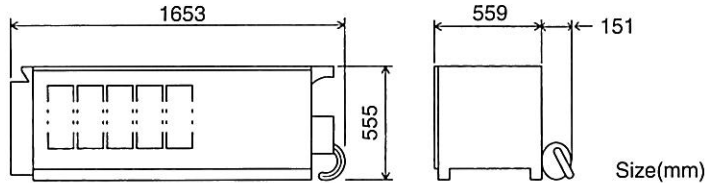
★ Condensing unit
